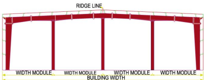
■ BEAM COLUMN - 3* (BC3) Note: *Denotes number of columns
