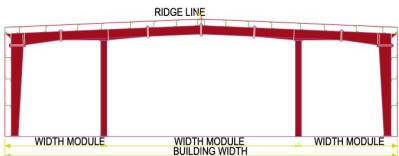
■ BEAM COLUMN - 2* (BC2)
