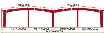
■ MULTI GABLE - 2 (BC1+BC1)
